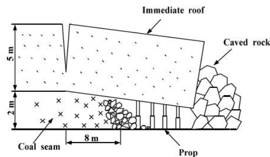
a. Roof fracture and rock burst
