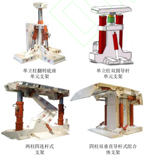
图 21 超前支护防冲支架 Fig. 21 Advance support anti-impact support
