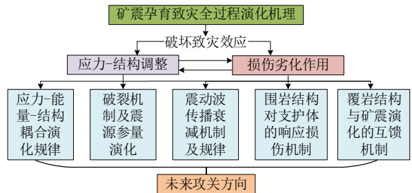
图 23 矿震孕育致灾全过程演化机理难题 Fig. 23 Difficult problem of evolution mechanism of the whole process of disaster-induced by mining tremors
