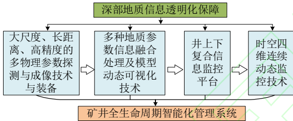
图 24 深部地质信息透明化保障难题 Fig. 24 Difficult problem of guarantee the transparency of deep geological information
