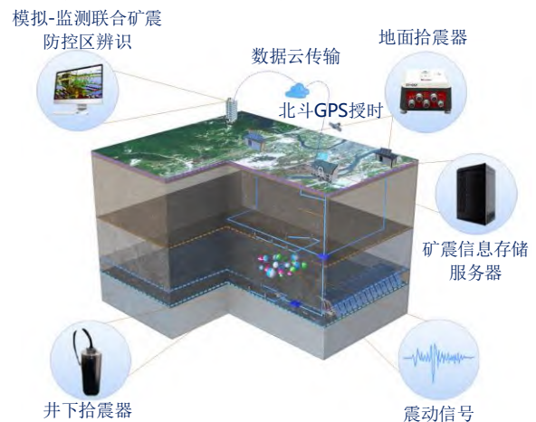
图 20 井地联合矿震系统示意图 Fig. 20 Schematic diagram of the combined well-ground mining tremors system
