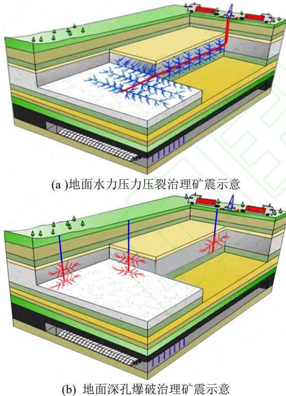
图 19 地面水力压裂和地面深孔爆破治理矿震 Fig. 19 Ground hydraulic fracturing and ground deep hole blasting for mining tremors control
