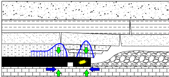
图5 煤体失稳诱发矿震的概念模型 Fig. 5 Conceptual model of coal mass instability induced mining tremors
