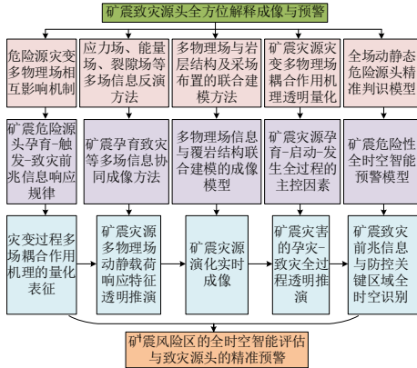
图 26 矿震致灾源头全方位解释成像与预警难题 Fig. 26 Difficult problem of comprehensive interpretation imaging and early warning of mining tremors source
