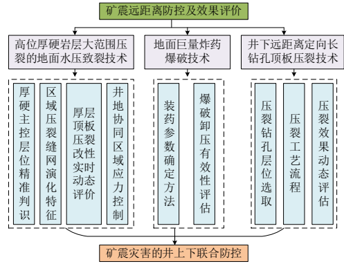
图 27 矿震远距离防控及效果评价难题 Fig. 27 Difficult problem of remote control and effect evaluation of mining tremors
