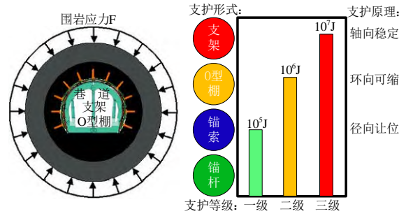
图 22 三级支护原理示意 Fig. 22 Schematic principle of three-stage support
